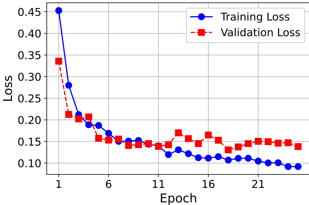
Training Loss Progress
